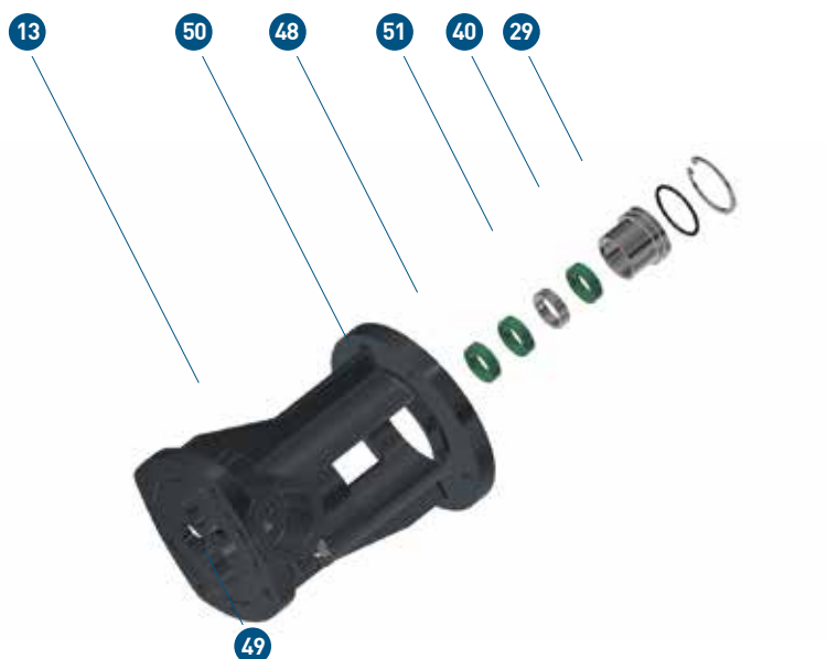
Fig. 309 - Lip seal details
