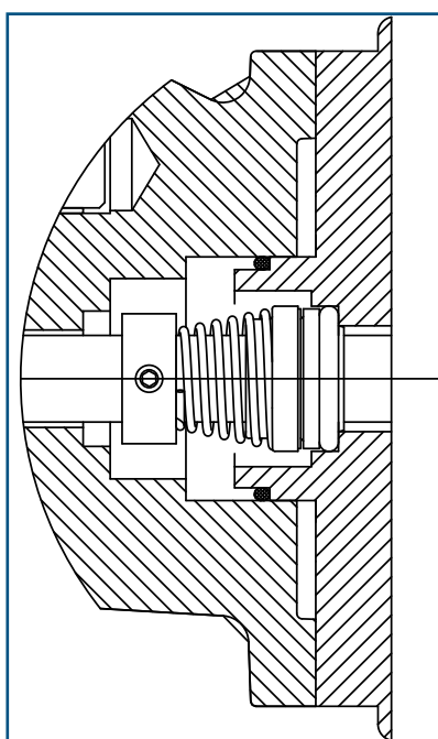
Fig. 405 – Mechanical seal
