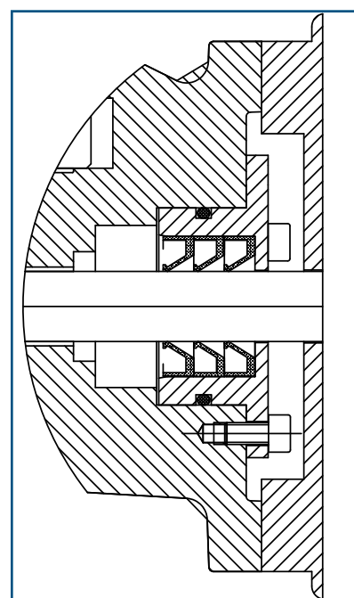
Fig. 406 – Lip seal
