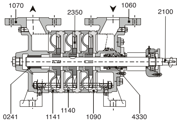
Design A (only for sizes 1100 up to 5100)
